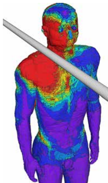
Figure D14 — Example 2: Induced electric field distribution from exposure to a 50 Hz wire positioned near the head.
